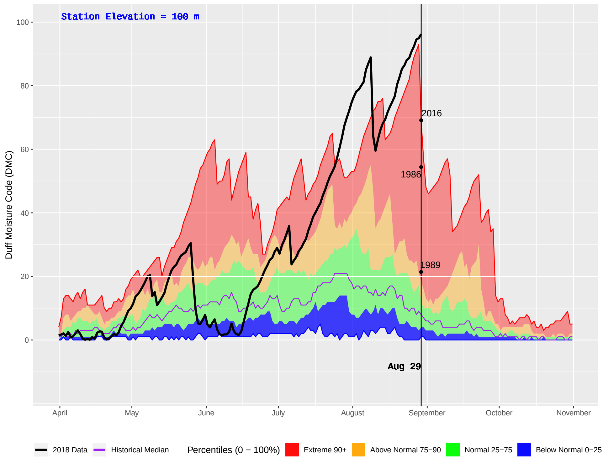
HONNA (93) : Historical (1986–2016) and Current (2018) Daily Duff Moisture Code (DMC)
